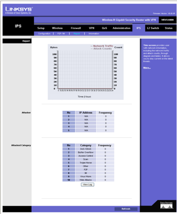
Figure 6-60: IPS - Report
